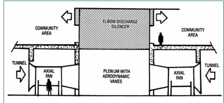
Schematic elevation of silencing system.
