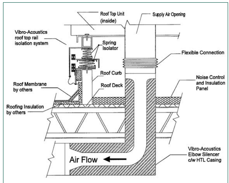
Vibro-Acoustics' noise and vibration control package was designed to meet the project's critical specifications.
