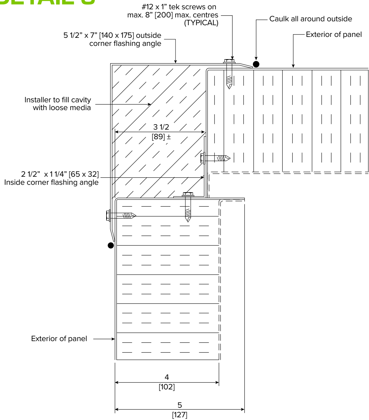
CORNER CONNECTION
