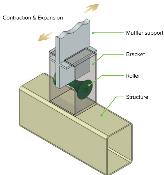
Fig. 1 Muffler support solution
